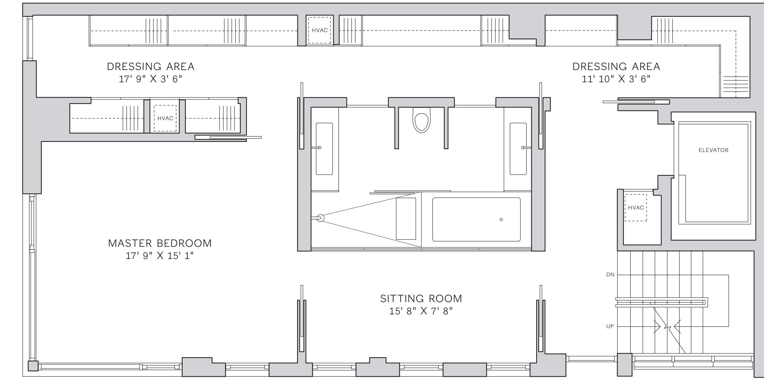
Third Level
